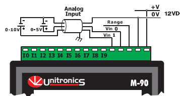
Analog-In Wiring
