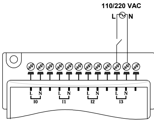
Input wiring (top group of inputs)
