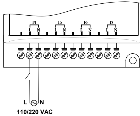
Input wiring (bottom group of inputs)
