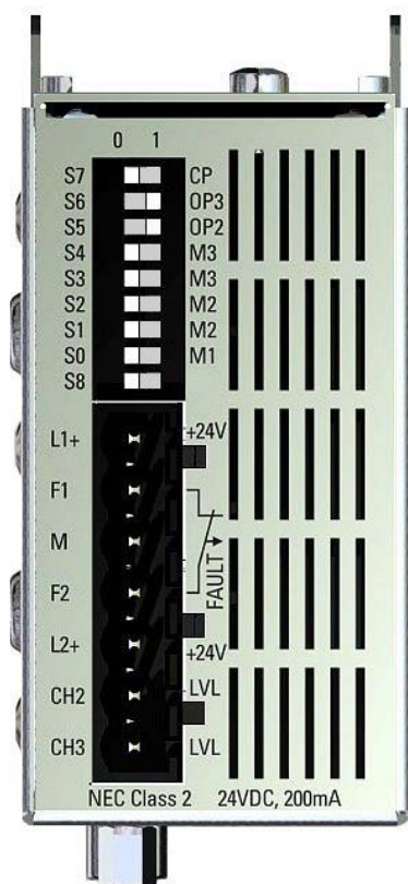
Figure 4-1 View of the OLM module from the top
