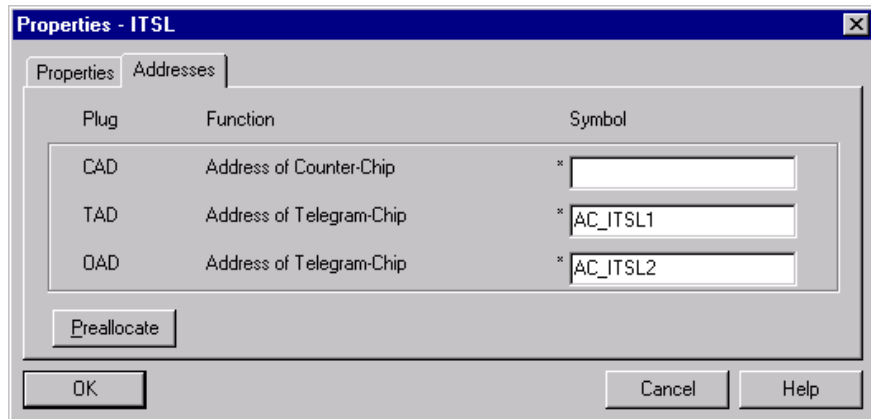
Fig. 3-65 Setting hardware addresses for an ITSL module with optional SLB module
