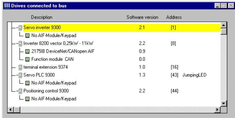
Abb. 8 Window Drives connected to bus
