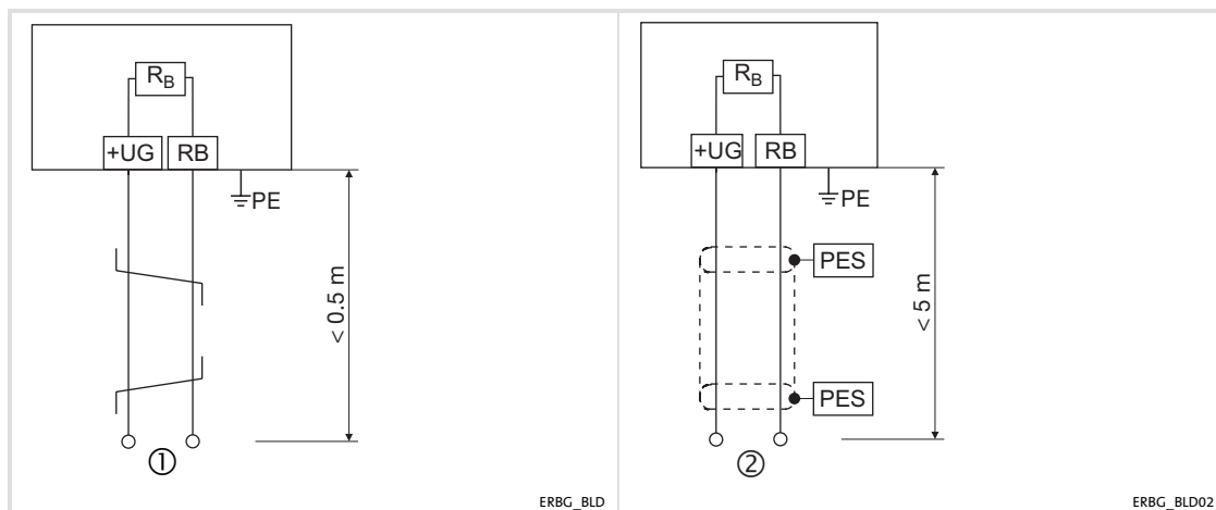
Fig. 8-2 Wiring of a brake resistor to the controller
