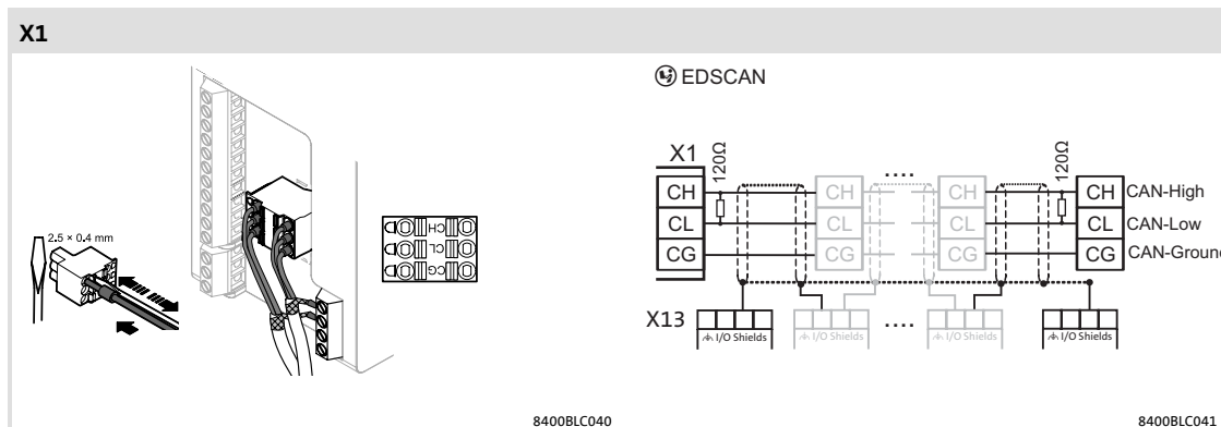
Fig. 6-16 CANopen connection
