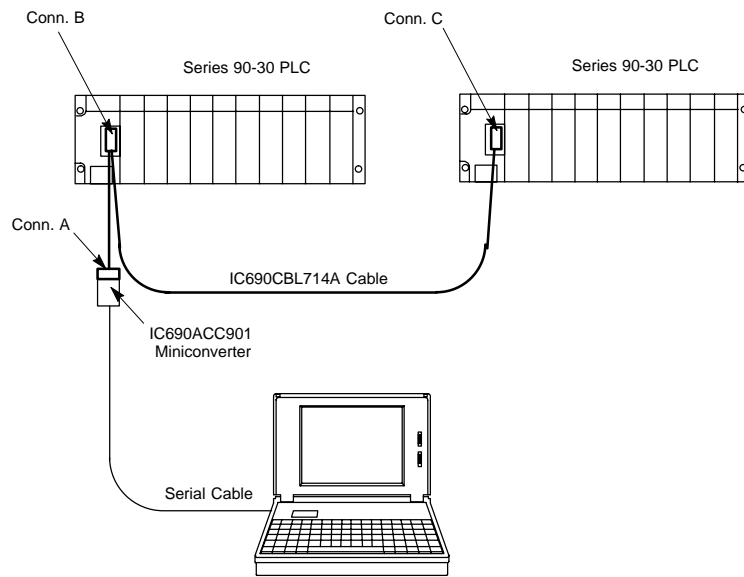
Figure 10-12. Multidrop Arrangement for Series 90-30 Redundant System
