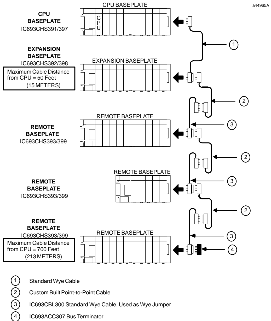
Figure 3-13. Example of Connecting Expansion and Remote Baseplates
