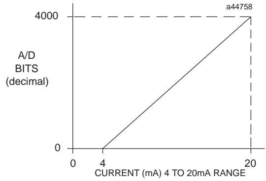
Figure 10-15. A/D Bits vs. Current Input for IC693ALG223
