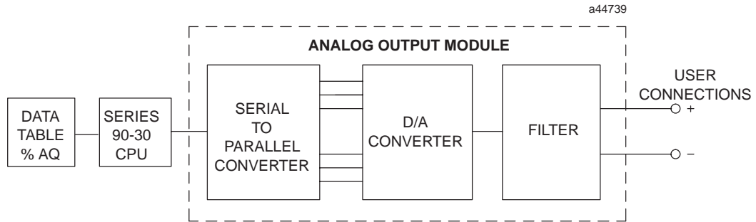
Figure 9-4. Analog Output Block Diagram
