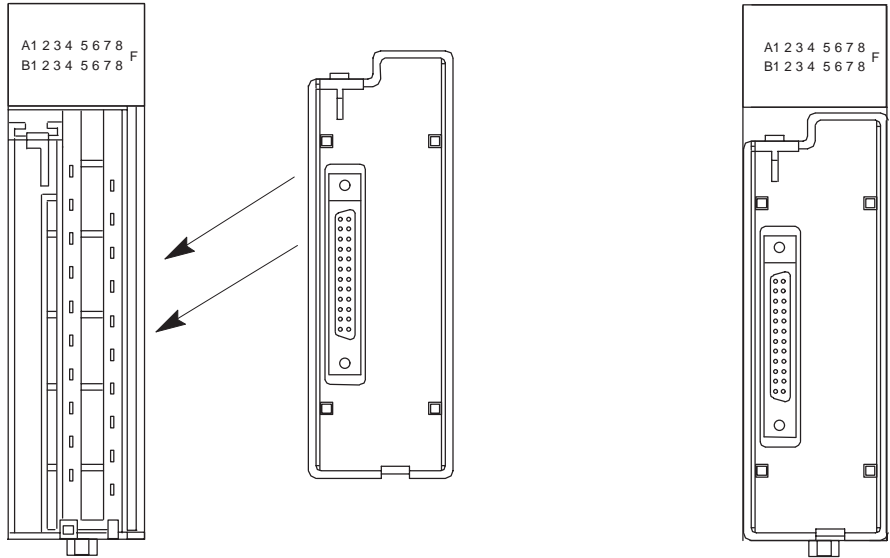
Installing the IC693ACC334 I/O Face Plate
