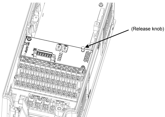
Figure 3.3 Mounting Completed
