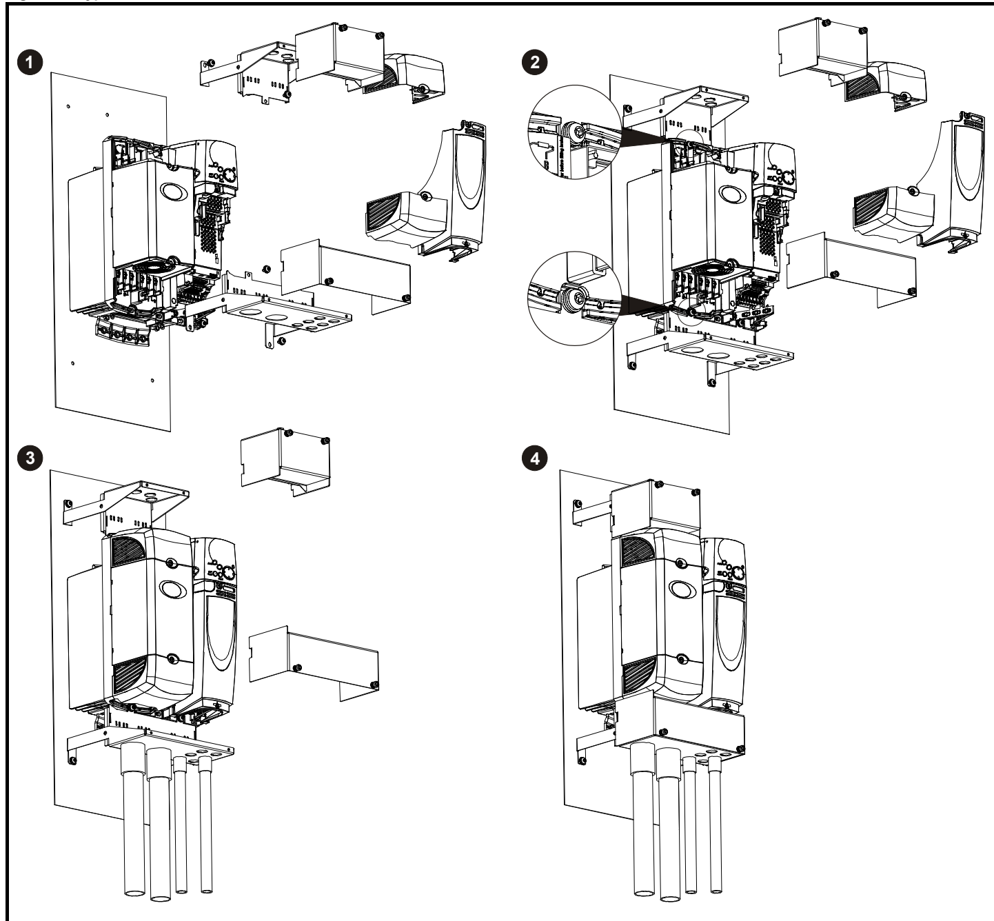
Figure 1 Typical installation for size 3 conduit connection box
