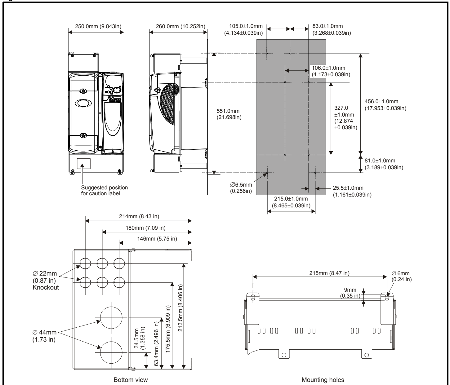
Figure 2 Dimensions of size 3 drive with conduit connection box fitted
