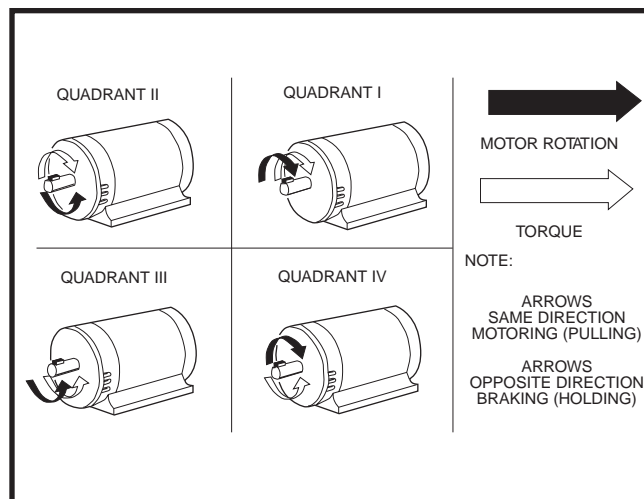
FIGURE 2. Four-Quadrant Drives
