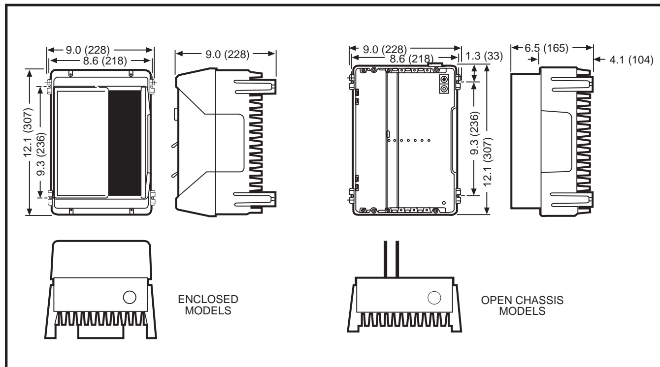
FIGURE 9. Series 2240 dimensions
