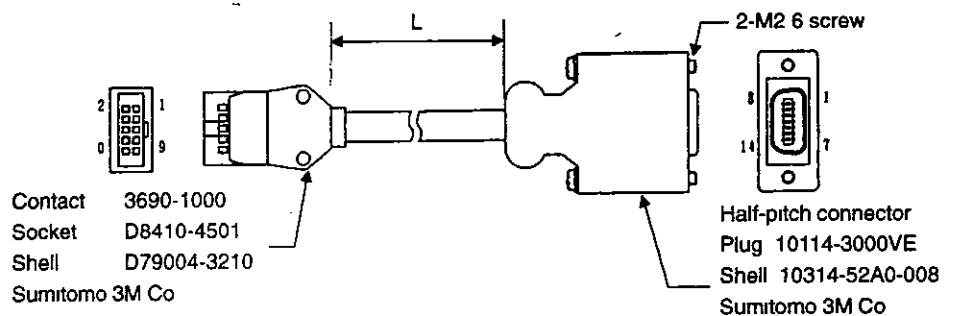
Figure 5 2 Cable Diagram
