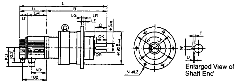
Figure 4.14 Larger Grease Lubricating Type
