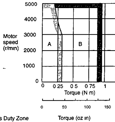
SGMAH-01B
