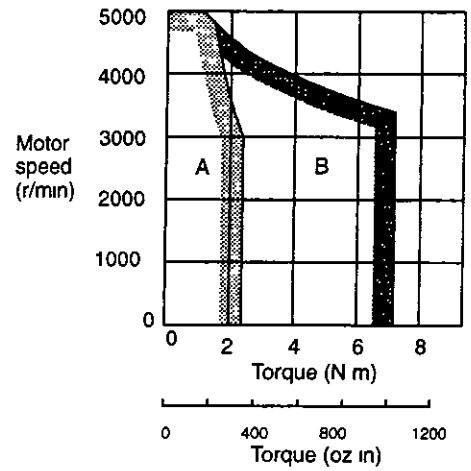
SGMPH-08A
