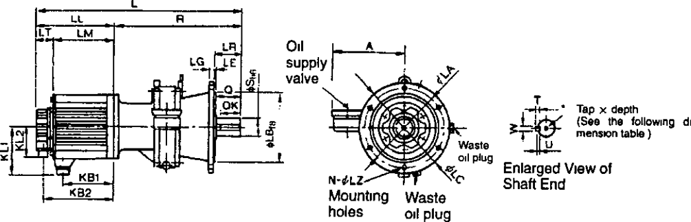
Figure 4.4 Smaller Oil Lubricating Type
