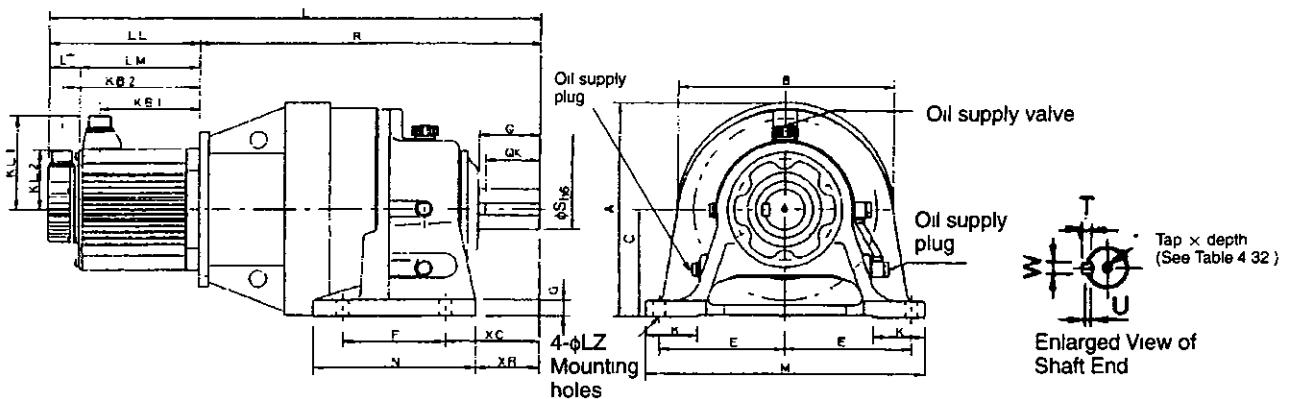
Figure 4.2 Oil Lubricating Type
