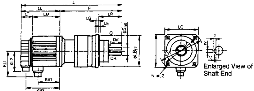
Figure 4.6 Smaller Grease Lubricating Type
