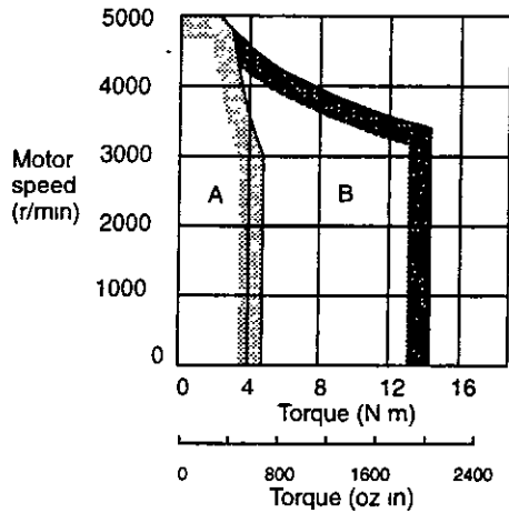
SGMPH-15A
