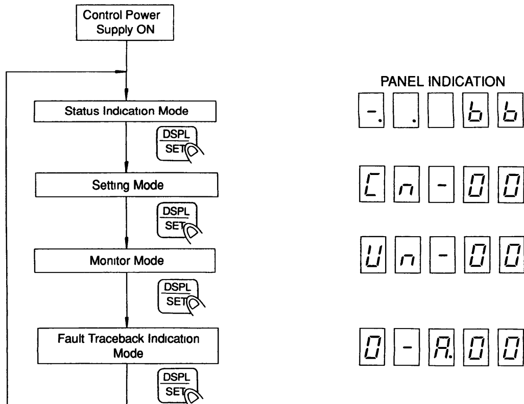
Fig 8.2 Mode Changeover
