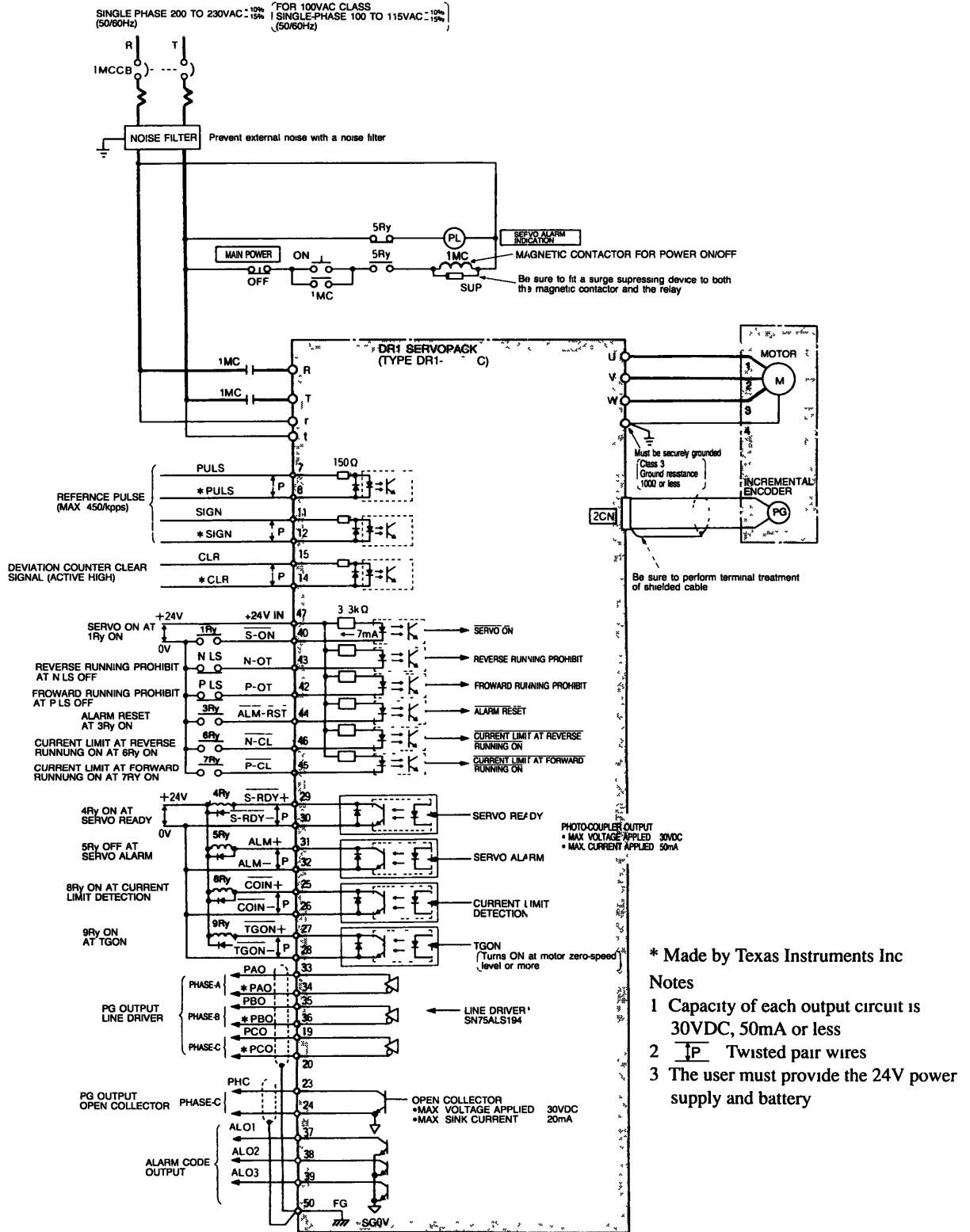
Fig 5.5 Example of Connection Diagram of DR1 SERVOPACK with a SERVOMOTOR and Peripherals
